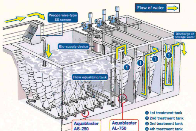
■ Basic flow diagram / Sewage water discharge
